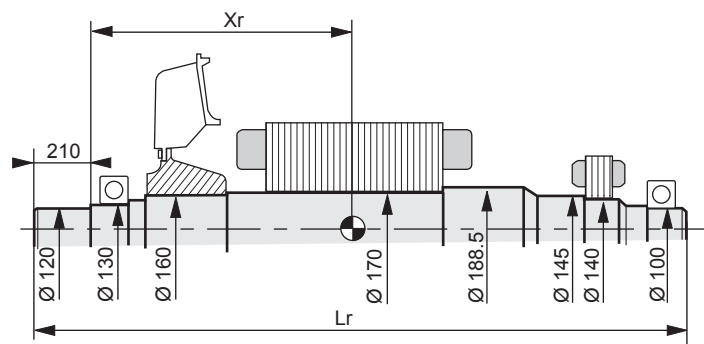
Centre of gravity: Xr (mm), Rotor length: Lr (mm), Weight: M (kg), Moment of inertia: J ( \text{kgm}^2 ): ( 4J = MD^2 )
